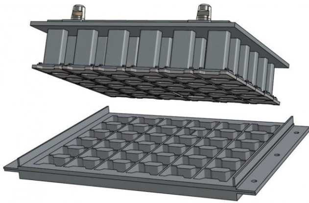
Mold and tamper assembly | product illustration
